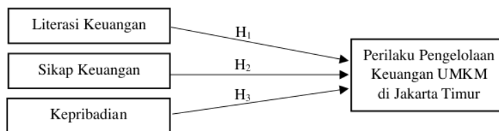
Gambar 1. Model Penelitian
