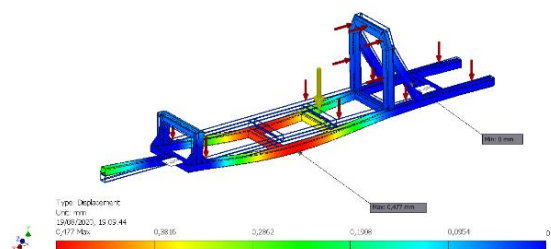
Gambar 6. Displacement
