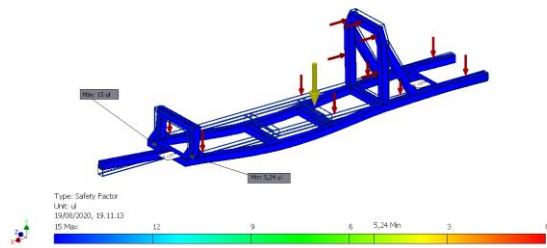
Gambar 7. Safety Factor
